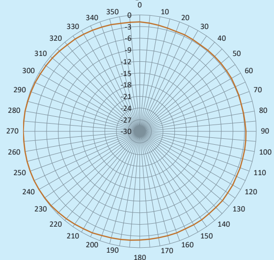
Beam Pattern @45 KHZ
